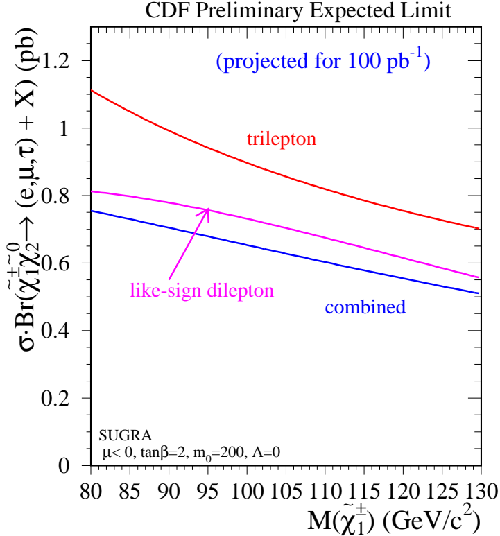
FIG. 2. Average expected limit on \sigma \cdot \mathcal{B} as a function of M_{\tilde{\chi}_1^\pm} for the LSD analysis, tripleton analysis, and the combination of both analyses. The parametrized efficiencies shown in Figure 1 are used along with the expected background from Monte Carlo in this calculation.
