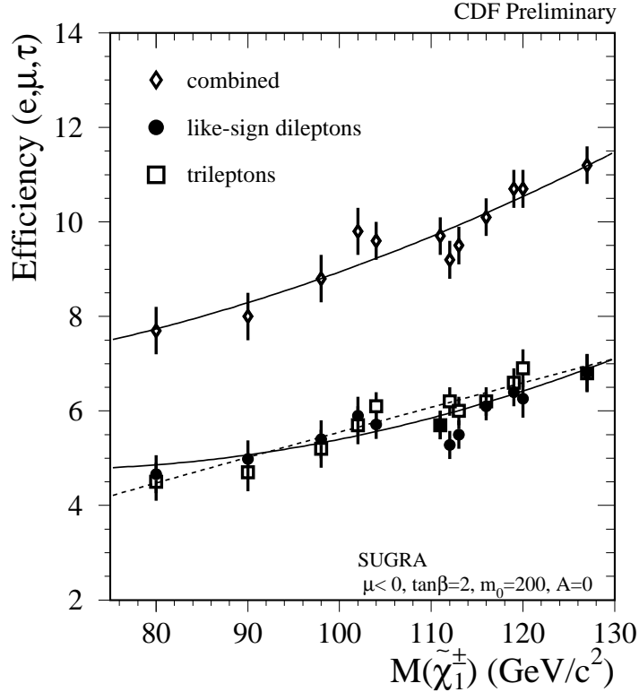
FIG. 1. The efficiency (as the percentage of events selected) for the trilepton, LSD, and combined analyses as a function of chargino mass. SUGRA parameters of \mu < 0, \tan \beta = 2, A_0 = 0, m_0 = 200 \text{ GeV}/c^2 , and m_{1/2} = 90 - 140 \text{ GeV}/c^2 were used to measure the efficiency.
