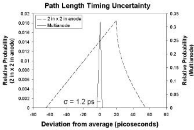
Fig. 4. The timing distribution resulting from path length differences on the anode. On a 2 in x 2 in anode, the RMS is as severe as 48 ps, but a multianode design improves the RMS to 1.2 ps.
