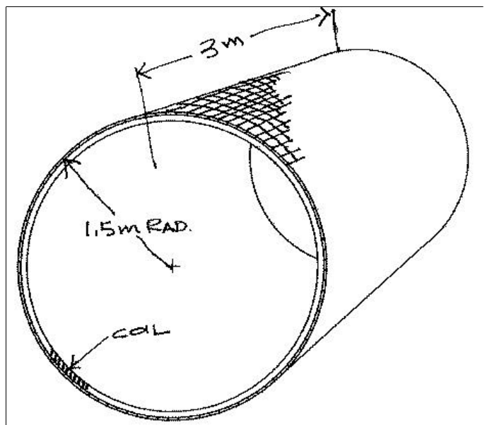
Fig. 2. A schematic showing the placement of photodetectors around a detector solenoid coil. The detectors may also be placed just inside of the coil.
