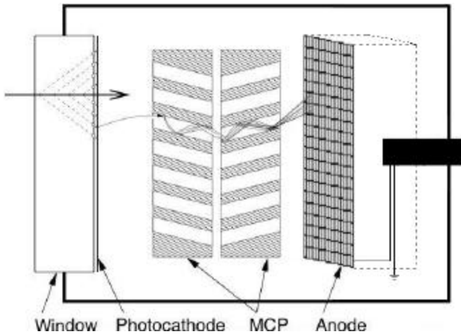
Fig. 3. A schematic of the proposed detection scheme. A relativistic particle produces Cherenkov radiation in the window of a PMT-MCP. This radiation is converted into electrons by a photocathode. The electrons produce a shower in the micro-channel plates, and the shower is deposited on the anode. After transmission through an impedance matched segment, the signal is detected from a central collector, and conveyed to an on-board chip in which it is digitized.
