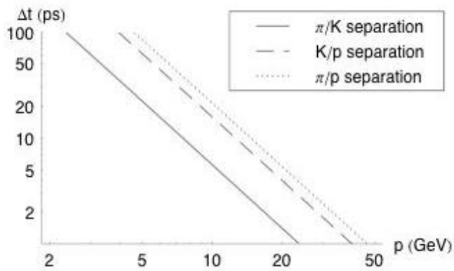
Fig. 1. The separations of pions, kaons, and protons, the difference in the time it takes two different particles with the same momentum to travel 1.5 m, as a function of momentum. Large time-of-flight detector systems have a time resolution on the order of 100 ps [2]-[4].
