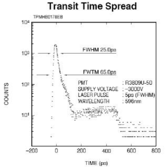
Fig. 5 The transit time spread for a single photo-electron event in Hamamatsu's MCP PMTs (taken from [10]). We approximate TTS in simulation as a Gaussian random variable with FWHM 25 ps.
