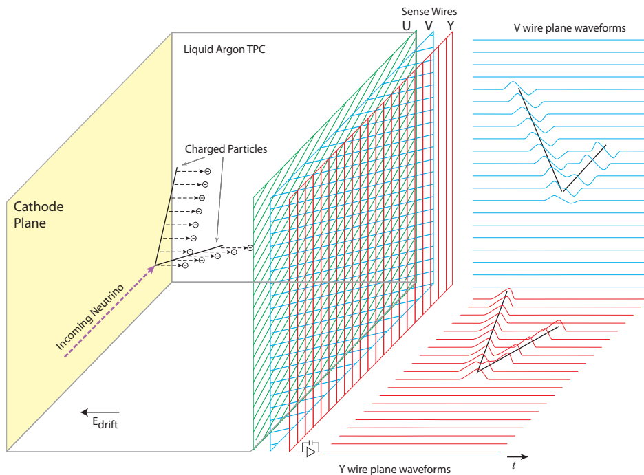
Figure 2. Operational principle of the MicroBooNE LArTPC.
