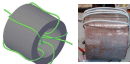
Saturable Inductor Model and Install
