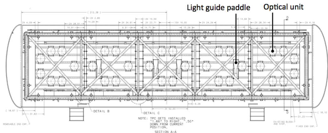
Figure 26. The MicroBooNE light collection system consists of a primary system of 32 optical units and a secondary optical system of four lightguide paddles [40]. These are mounted behind the anode wire planes such that the view is not obscured by structural cross bars of the LArTPC.
