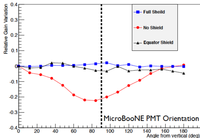
Figure 34. Red: angular dependence of a PMT response with no shield; black: for a shield that reaches the tube equator; blue: for a shield that fully covers the tube to the zenith.
