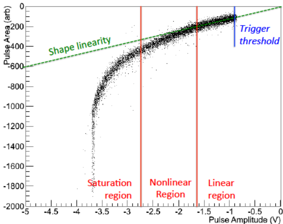
Figure 37. As shown by the VST, linearity of cosmic-ray induced PMT pulses is maintained up to amplitudes of around -1.7 V (300 PE), and amplitude saturation occurs at -3.7 V (670 PE) [50].
