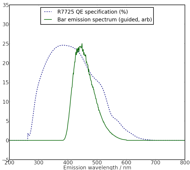
Figure 39. Measured emission spectra of the light guide coating in guided mode, and the R7725 quantum efficiency. Only the quantum efficiency of the non-undercoated PMT model is shown, from [71].
