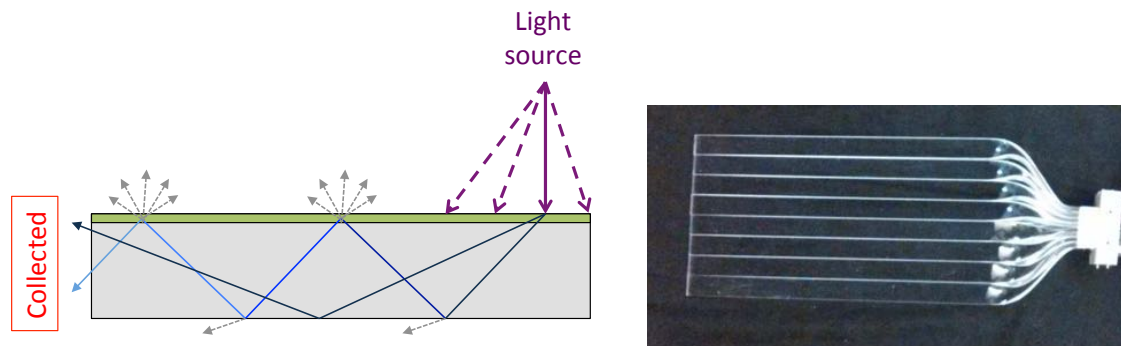
Figure 38. Left: illustration of guiding mode, used by the paddles. Right: photograph of a coated paddle.
