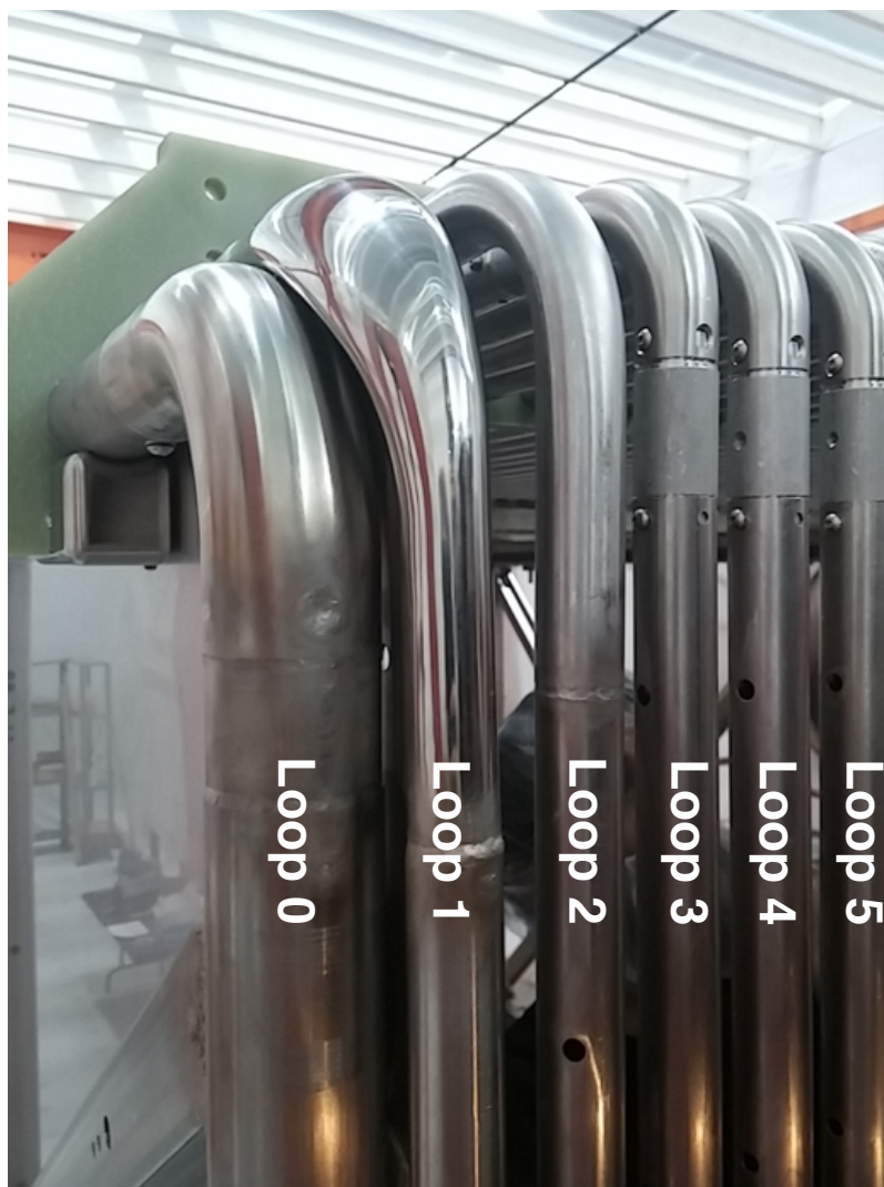
Figure 12. Photograph of the field cage during construction, with loops 0 (cathode) through 5 labeled. Field cage loops closest to (and including) the cathode are modified to reduce sharp edges that would result in higher electric fields.
