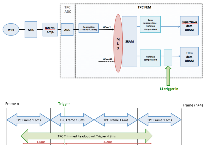
Figure 56. MicroBooNE trigger readout.
