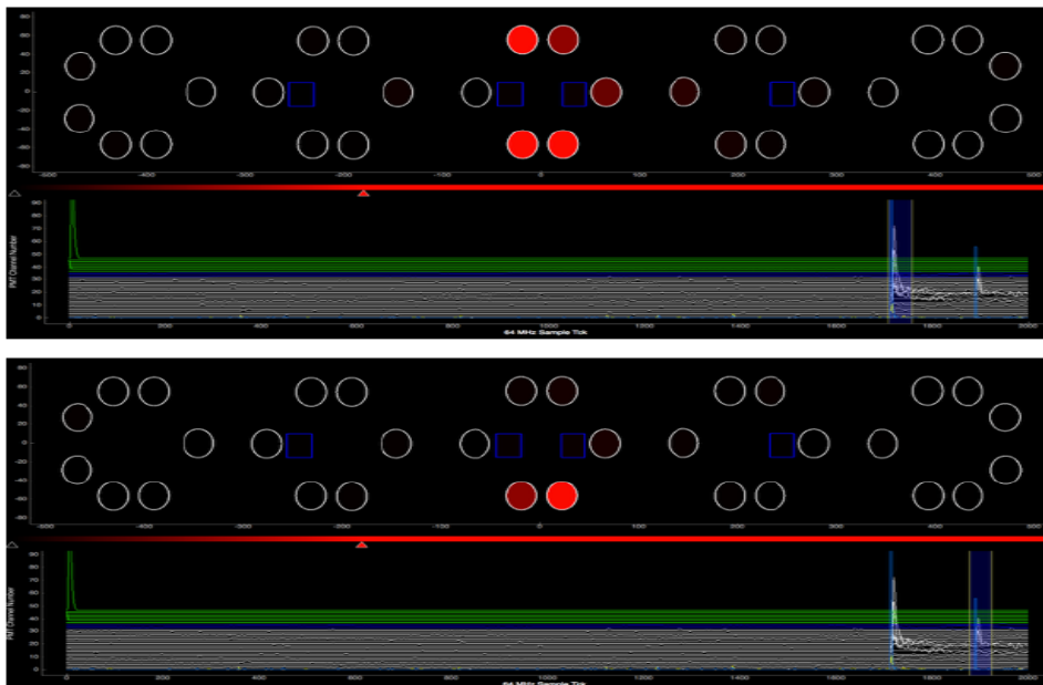
Figure 27. Displays showing two sequential events in the argon as seen by the light collection system. The sequence is consistent with a muon that stops (top) and decays (bottom). The circles correspond to the optical units. Red circles indicate those units with hits within the time range indicated by the vertical bars drawn on the PMT waveforms, which are shown at the bottom of each display.
