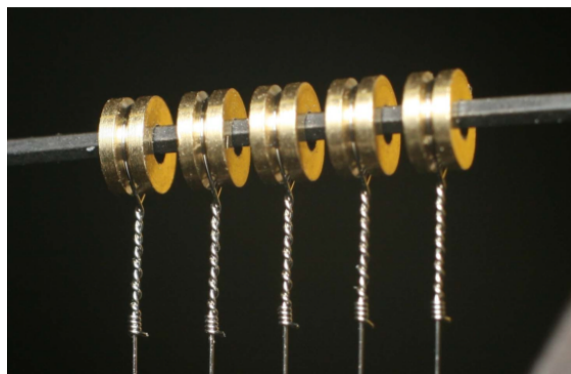
Figure 18. Photograph of the wire termination on the brass ferrules. Each ferrule is 3 mm in diameter, and 1.5 mm thick.
