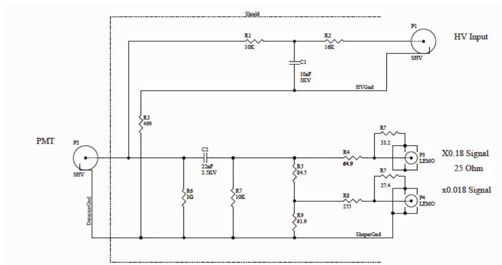
Figure 36. The “splitter” circuit. The circuit connects the HV source to the PMT. It also provides a pathway for signal pulses from the PMT to reach the readout electronics via an AC-coupling capacitor (C2). The signal is split into two copies, one provided with an attenuation factor of 0.18 and another at 0.018. Both signal sources are recorded by the readout electronics in order to provide two dynamic ranges.
