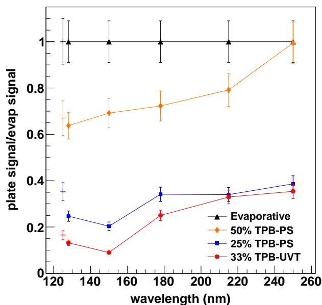
Figure 32. Measured efficiencies of various wavelength-shifting coatings, from [62]. In this plot, 50% TPB-PS is the MicroBooNE plate coating used in the optical units. The 33% TPB-UVT is the light guide coating for the secondary light collection system described below. Connected points were measured in a vacuum monochromator at room temperature, and non-connected points were measured in liquid argon with 128 nm scintillation light. All points are normalized to the performance of an evaporatively coated plate.
