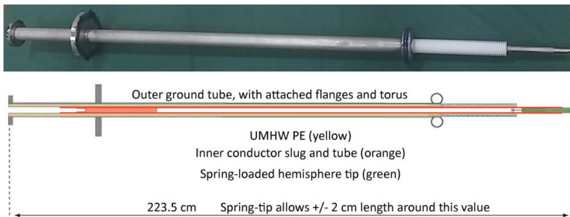
Figure 24. Photograph and drawing of the production HV feedthrough. The spherical probe tip is attached to the end of the inner conductor, on the right side of these figures.
