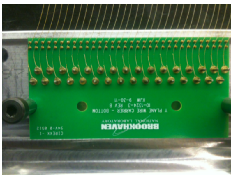
Figure 19. Photograph of a collection plane wire carrier board that has been filled with wires, but has not yet had the cover plate installed.
