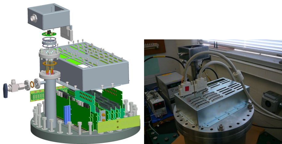
Figure 51. Left: diagram of the signal feedthrough assembly, which includes intermediate amplifiers, Faraday cage, bias-voltage feedthrough and filtering circuit. Right: photograph of one of the feedthrough assemblies, partially constructed and being tested.
