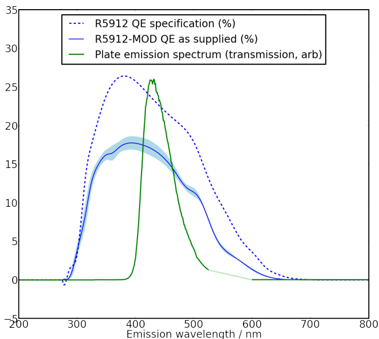
Figure 30. The specification for the non-platinum undercoated PMT from [56]. The blue band shows the mean and standard deviation of the four quantum efficiency curves provided by Hamamatsu for the installed PMTs. Also shown is the measured emission spectra of the MicroBooNE wavelength-shifting coatings, discussed in section 5.2.2 [50].
