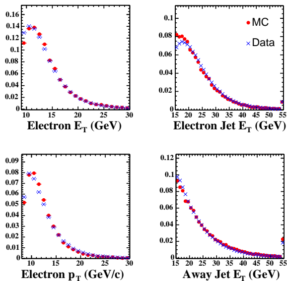
FIG. 2: Data/Monte Carlo comparison of some quantities of tagged electron jets ( L_{2D} > 0 , identified conversions have been removed for plotting purposes). Histograms are normalized to unit area. From top-left, clockwise: electron E_T , electron-jet E_T , away-jet E_T , electron p_T . (The last bin includes all overflow entries.)
