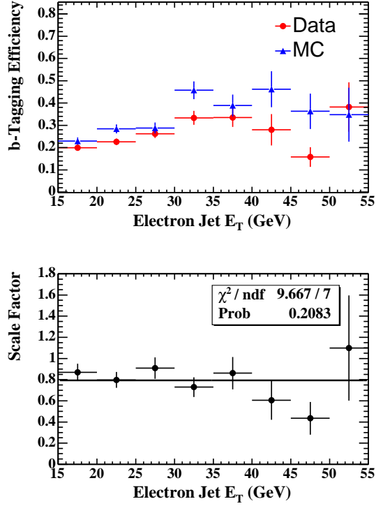
FIG. 6: Efficiency to tag a b -jet as a function of jet E_T in data and Monte Carlo (top), and data/MC scale factor (bottom). The scale factor is consistent with being constant over the E_T range investigated.
