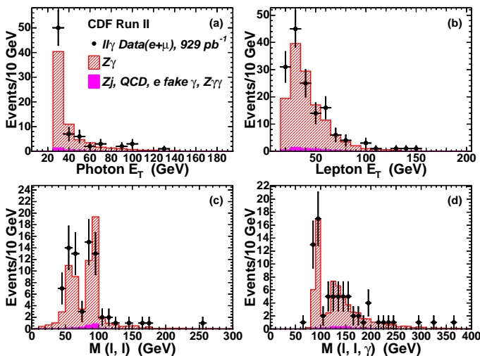
FIG. 7: The distributions for events in the \ell\ell\gamma sample (points in a) the E_T of the photon; b) the E_T of the leptons (two entries per event); c) the 2-body mass of the dilepton system; and d) the 3-body mass M_{\ell\ell\gamma} . The histograms show the expected SM contributions.
